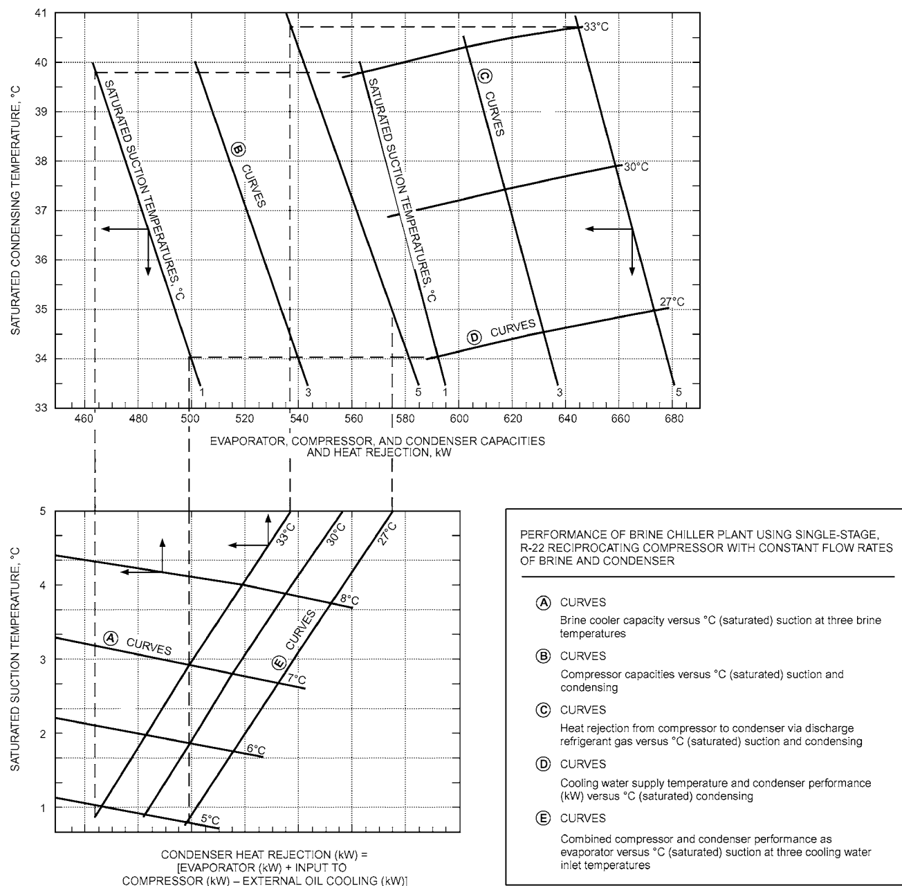
Fig. 1 Brine Chiller Balance Curve
